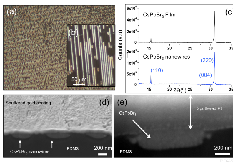
Fig. 3 Polycrystalline \text{CsPbBr}_3 nanowires characteristics. Optical images of \text{CsPbBr}_3 Perovskite nanowires obtained on (a) DVD and (b) CD replica PDMS substrates. (c) XRD pattern of \text{CsPbBr}_3 nanowires and of a \text{CsPbBr}_3 film structure. (d) FESEM image of a lateral view of a sample of \text{CsPbBr}_3 nanowires (obtained on PDMS replica of DVD structure) cut by FIB milling perpendicularly to the surface and coated with sputtered gold. (e) FESEM image of the cross section of a \text{CsPbBr}_3 nanowire grown on PDMS replica of CD structure (Sputtered Pt coating was used to cover the sample before the FIB milling)
