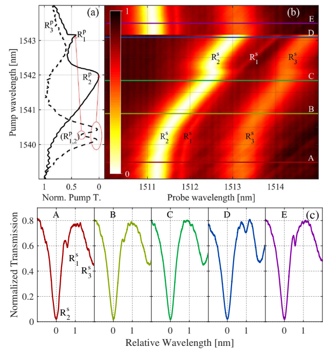
Fig. 6. Results of the pump and probe experiment. Panel (a) shows the cold (dashed) and hot (solid) cavity transmission spectra of the device around the strongly pumped resonance doublet. The thermo-optic nonlinearity, induced by the pumped doublet, also affects the other resonances (b), allowing for a relative detuning of the peaks as shown by the transmission color map. (c) Selected transmission spectra show the transformation of the Fano resonance in the vicinity of the critical phase point, where a complete disappearance of the R_1^s peak feature takes place (panel C). The probe spectrum time-evolution, together with the pump dynamic transmission is represented in Visualization 1.
